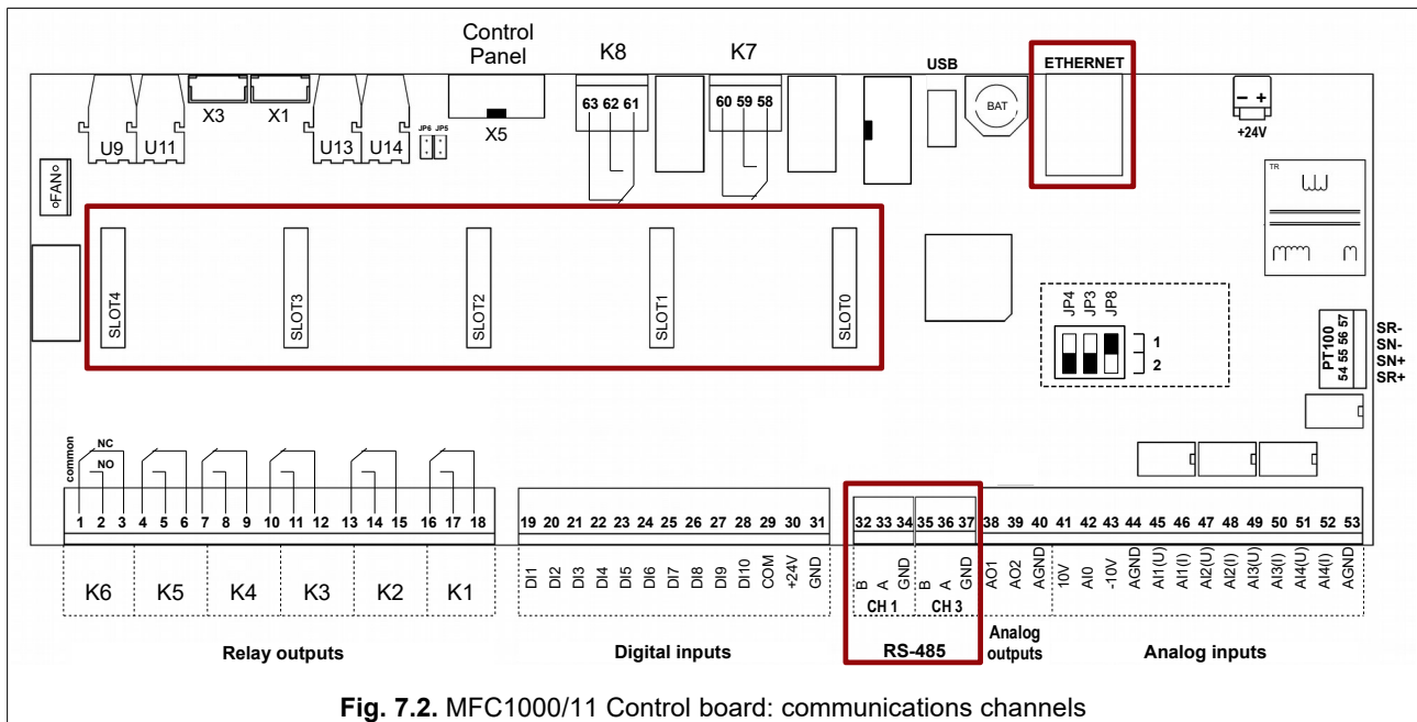
Fig. 7.2. MFC1000/11 Control board: communications channels
